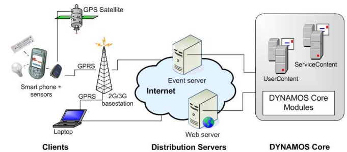
Fig. 3. The DYNAMOS overall reference architecture
