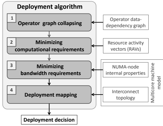
Figure 4: Overview of the deployment algorithm
