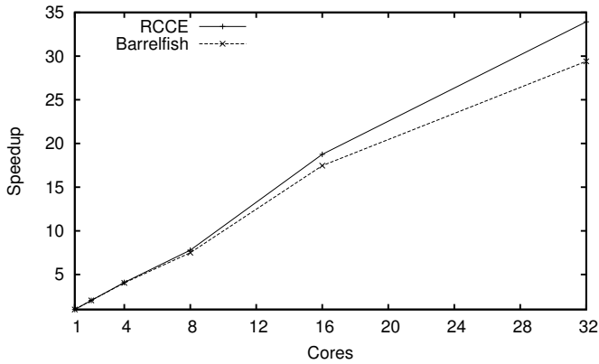
Fig. 4. RCCE LU benchmark speedup comparison
