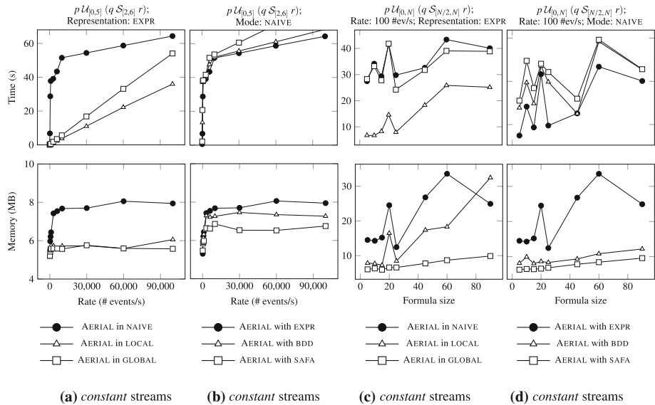
Fig. 7 Time (top) and memory (bottom) usage of AERIAL MDL’s modes and representations
