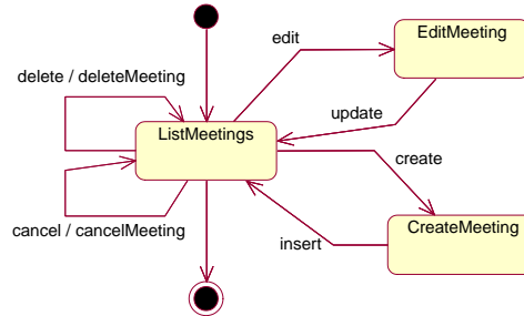
Figure 2. Scheduler Application Statechart
