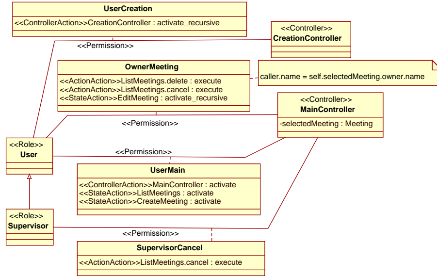
Figure 13. Policy for Scheduling Application
