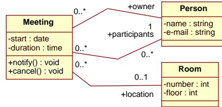
Figure 1. Scheduler Application Class Diagram
