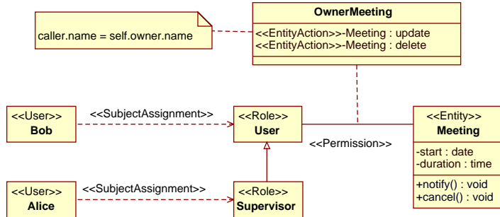
Figure 5. Example of the Concrete Syntax of SecureUML
