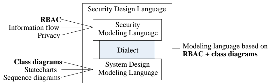
Figure 3. Security Design Language Schema
