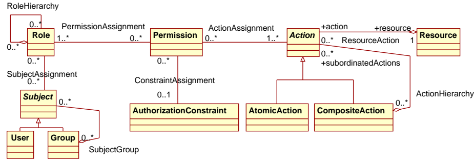
Figure 4. SecureUML Metamodel
