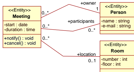
Figure 7. Scheduling Application
