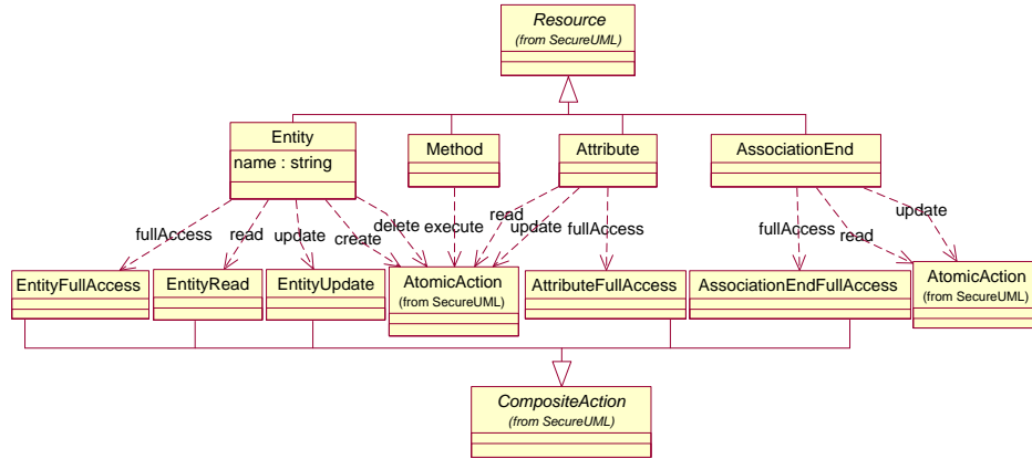
Figure 8. SecureUML Dialect for ComponentUML Metamodel
