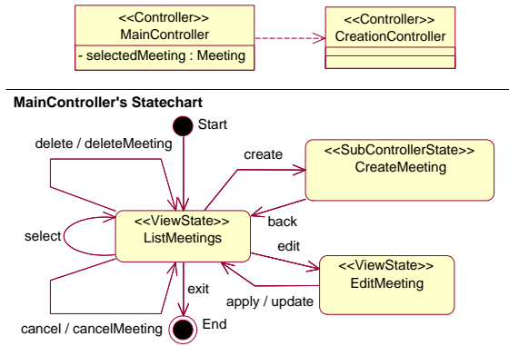
Figure 11. Controllers for the Scheduling Application
