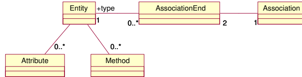
Figure 6. ComponentUML Metamodel
