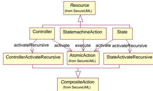
Figure 12. Resource Model of ControllerUML
