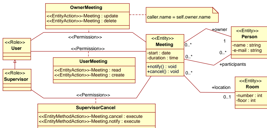
Figure 9. Scheduler Example with Authorization Policy
