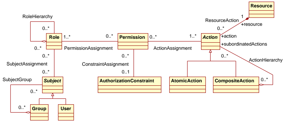
Figure 8: SecureUML metamodel
