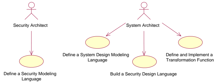
Figure 6: The roles and activities in the tool development process
