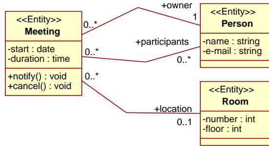
Figure 11: Scheduling application
