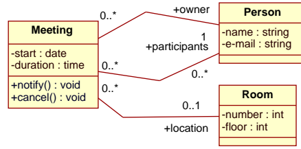
Figure 3: Scheduler application class diagram
