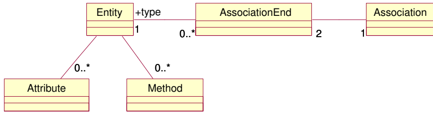
Figure 10: ComponentUML metamodel
