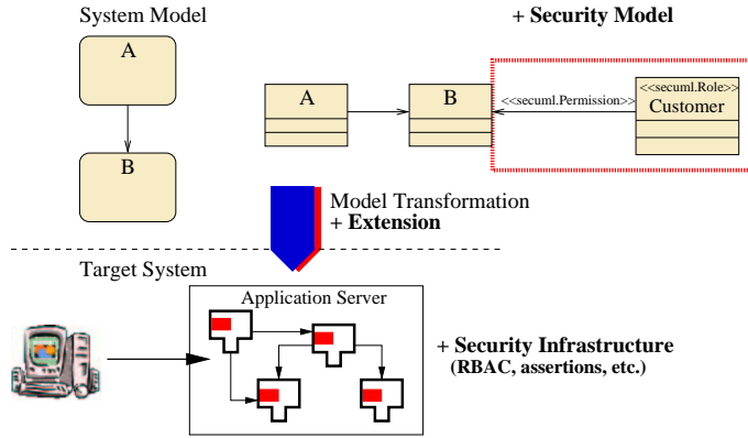
Figure 2: Model Driven Security
