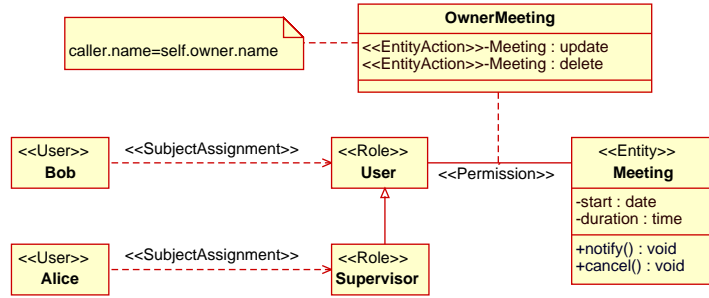
Figure 9: Example of the concrete syntax of SecureUML
