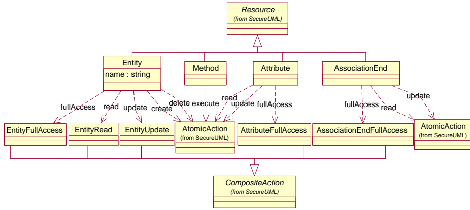
Figure 12: SecureUML dialect for the ComponentUML metamodel
