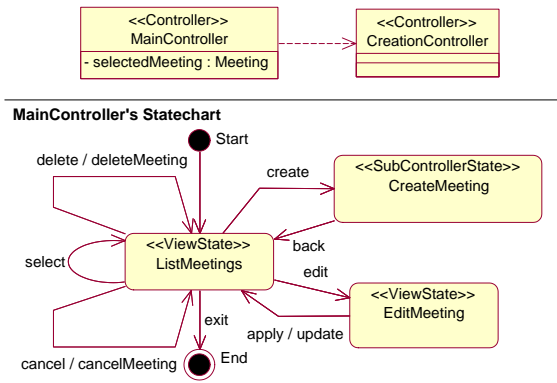
Figure 16: Controllers for the scheduling application
