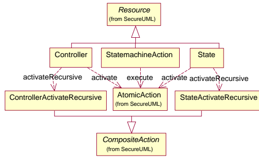
Figure 17: Resource model of ControllerUML
