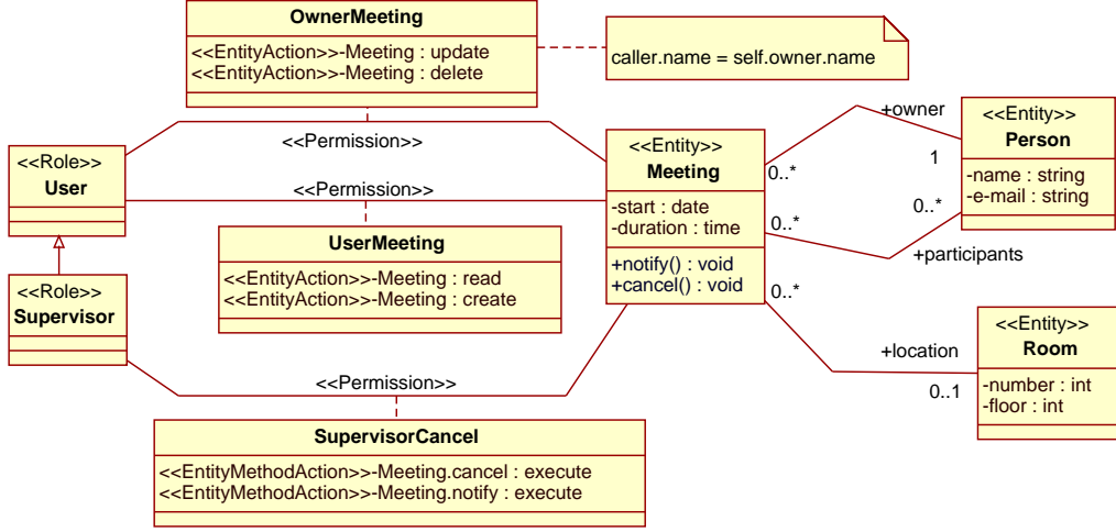
Figure 13: Scheduler example with authorization policy
