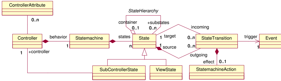
Figure 15: Metamodel of ControllerUML
