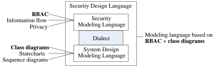
Figure 5: Security design language schema
