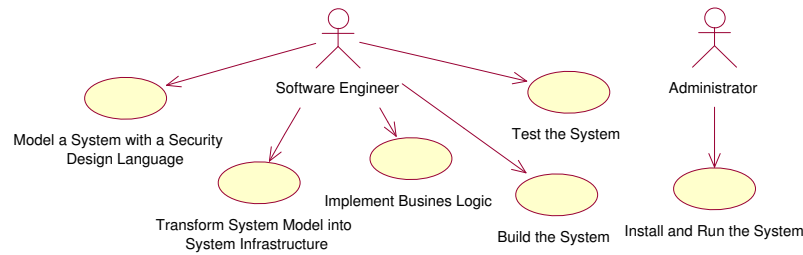
Figure 7: The roles and activities in the system development process
