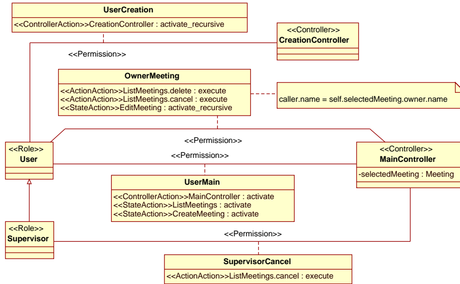
Figure 18: Policy for the scheduling application
