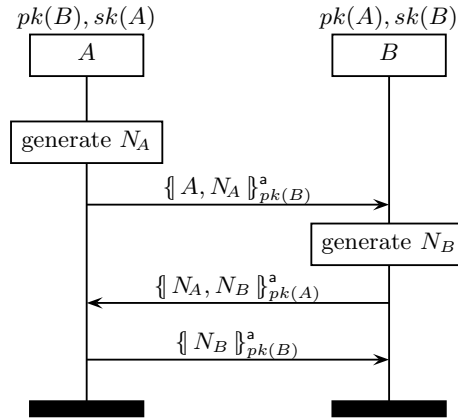
Fig. 24.1. Needham-Schroeder protocol (NS)
