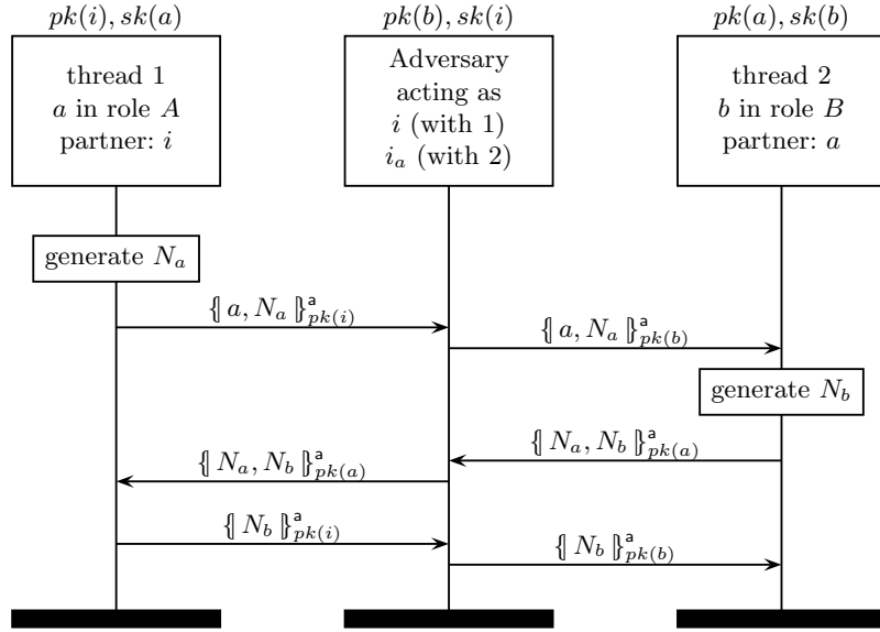
Fig. 24.2. Lowe's man-in-the-middle attack on the Needham-Schroeder protocol
