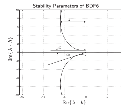
Figure: Stability parameters of a stiffly-stable algorithm
