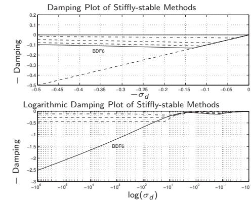
Figure: Damping plot of BDF6 and other 6 th -order stiffly-stable methods
