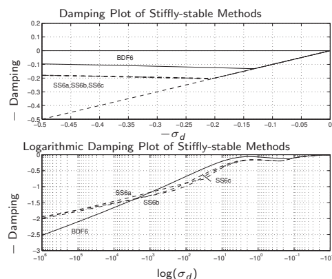
Figure: Damping plot of BDF6 and other 6 th -order stiffly-stable methods
