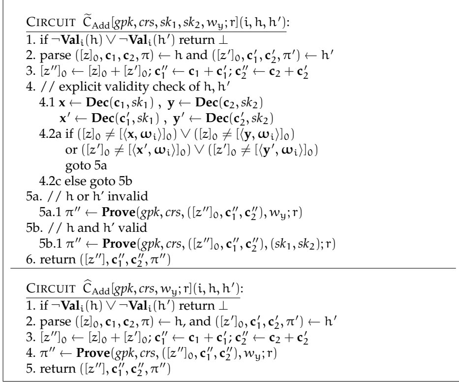
Figure 4: Circuits for addition of group elements used in Lemma 5.1. \hat{p} includes gpk = (pp_0, pk_1, pk_2, [W]_0, \text{TD}, \tilde{y}) where \tilde{y} \in \text{TD} (also includes a hiding CRS \widehat{crs}' ). Both circuits also have hard-coded (the) witness w_y to \tilde{y} \in \text{TD} . Top: sk_1, sk_2 are used to produce \pi'' on valid inputs. Bottom: w_y is always used to produce \pi'' .
