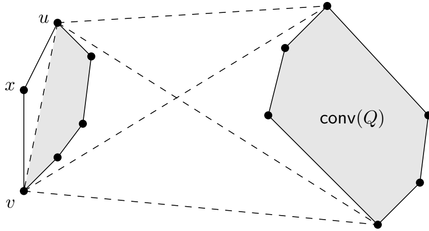
Figure 3.3: Where does x lie?
