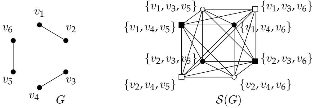
Figure 1.8: A counterexample for the converse of Lemma 1.17.
