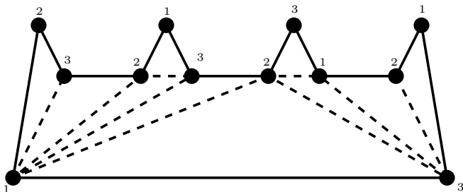
Figure 1.2: A polygon P with a triangulation and a vertex-3-coloring which can be guarded by 4 vertex-guards but not by 3.
