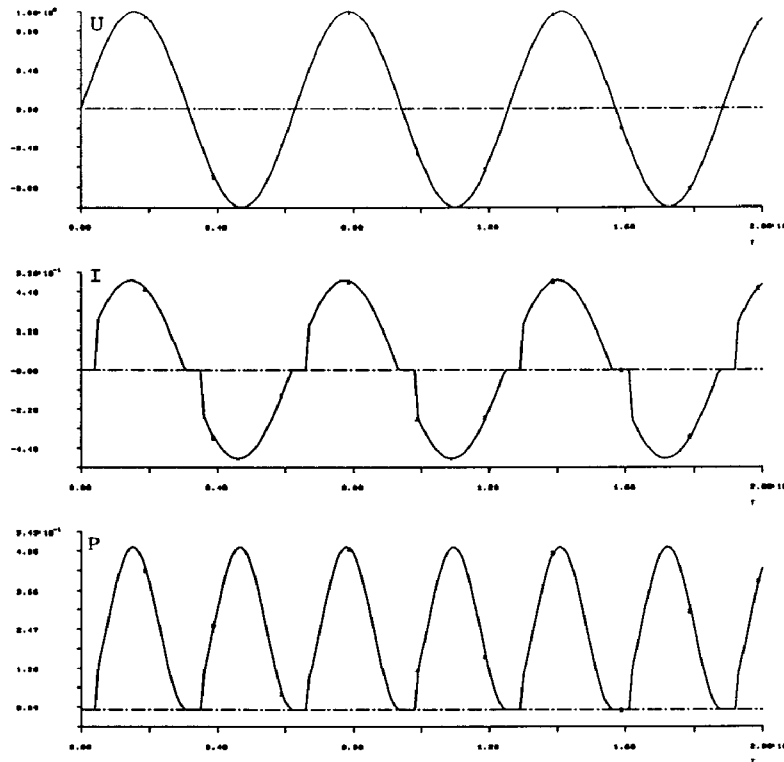
Fig. 1: AC-motor driven in phase cutting technique
