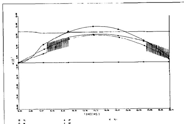
Fig. 4: Current as a function of simulated time
