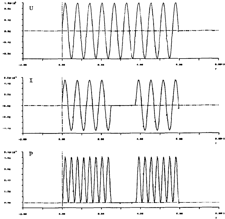
Fig. 2: AC-motor driven in burst technique
