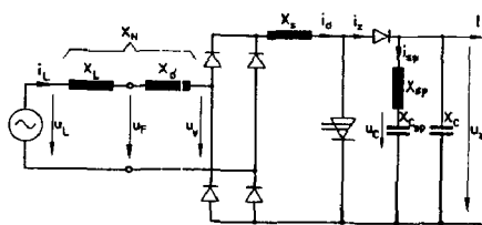
Fig. 3: AC-motor driven in chopper technique
