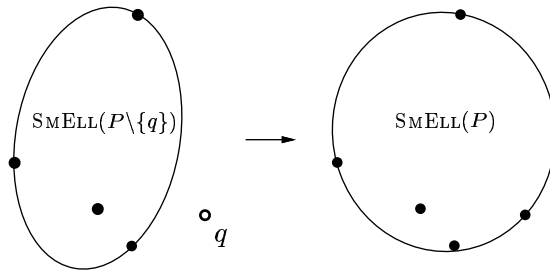
Figure 1: The inductive step in Welzl’s algorithm
