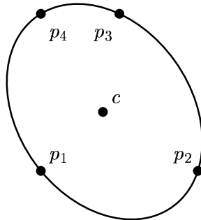
Figure 3: Irrational smallest ellipse through four points
