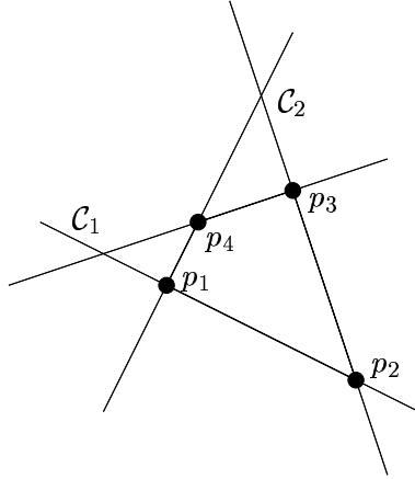
Figure 2: Two special conics through four points
