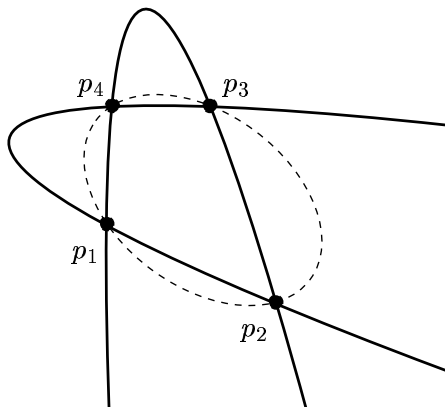
Figure 4: The two parabolas through four points
