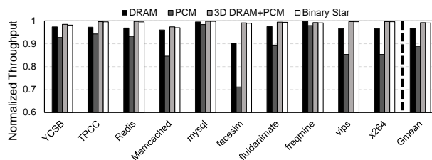
Figure 9: System performance of different memory configurations with no ECC and Binary Star. We normalize the throughput of each configuration to the throughput of 3D DRAM LLC with DRAM.
