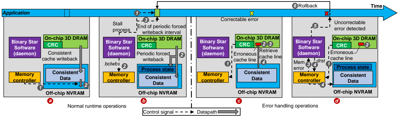
Figure 5: An example of running an application on Binary Star.
