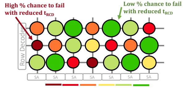
Figure 15: Key idea of D-RaNGe. Reproduced from [419].
