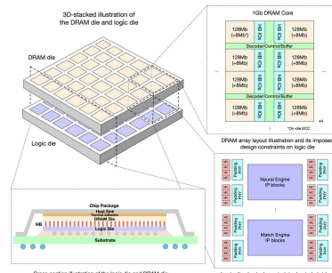
Figure 35: HB-PNM logic & DRAM dies and architecture. Reproduced from [515].
