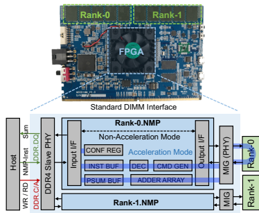
Figure 33: AxDIMM hardware architecture. Reproduced from [512].
