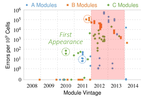
Figure 2: RowHammer vulnerability for DRAM modules manufactured between 2008 and 2014. Reproduced from [245]. Originally presented in [30, 246].
