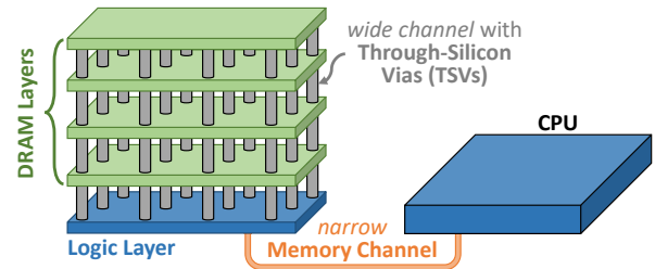
Figure 9: High-level overview of a 3D-stacked DRAM architecture. Reproduced from [341].
