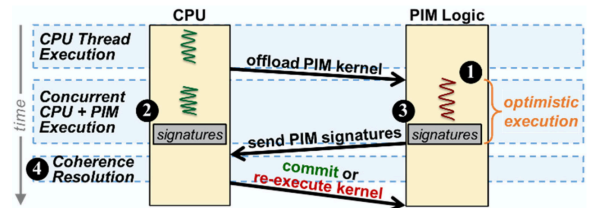
Figure 26: High-level operation of CoNDA, a new coherence mechanism for near-data accelerators, including PNM and PUM. Reproduced from [341]. Originally presented in [211].
