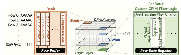
Figure 20: Left block: GRIM-Filter bitvector layout within a DRAM bank. Center block: 3D-stacked DRAM with tightly integrated logic layer stacked underneath with TSVs for high inter-layer data transfer bandwidth. Right block: Custom GRIM-Filter logic placed in the logic layer, for each vault. Reproduced from [130].
