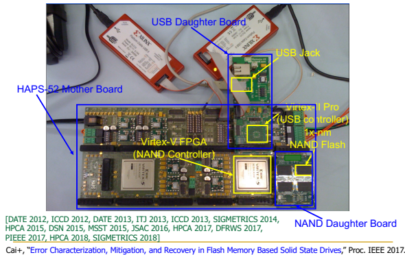
Figure 5: Example of an intelligent flash memory controllers. The figure depicts a picture of one of our real experimental infrastructures (from [308]) used for the design and evaluation of intelligent flash memory controllers. Reproduced from [26].
