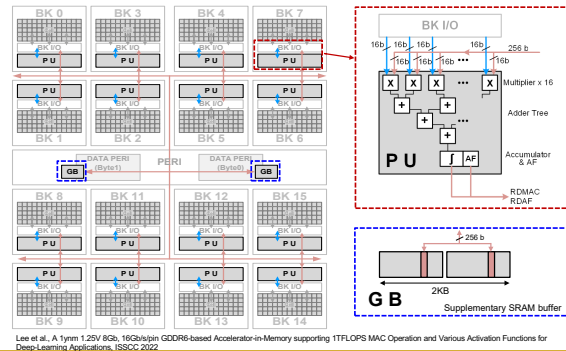
Figure 34: AiM system organization. Reproduced from [513].
