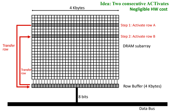
Figure 10: RowClone Fast Parallel Mode. Reproduced from [245].
