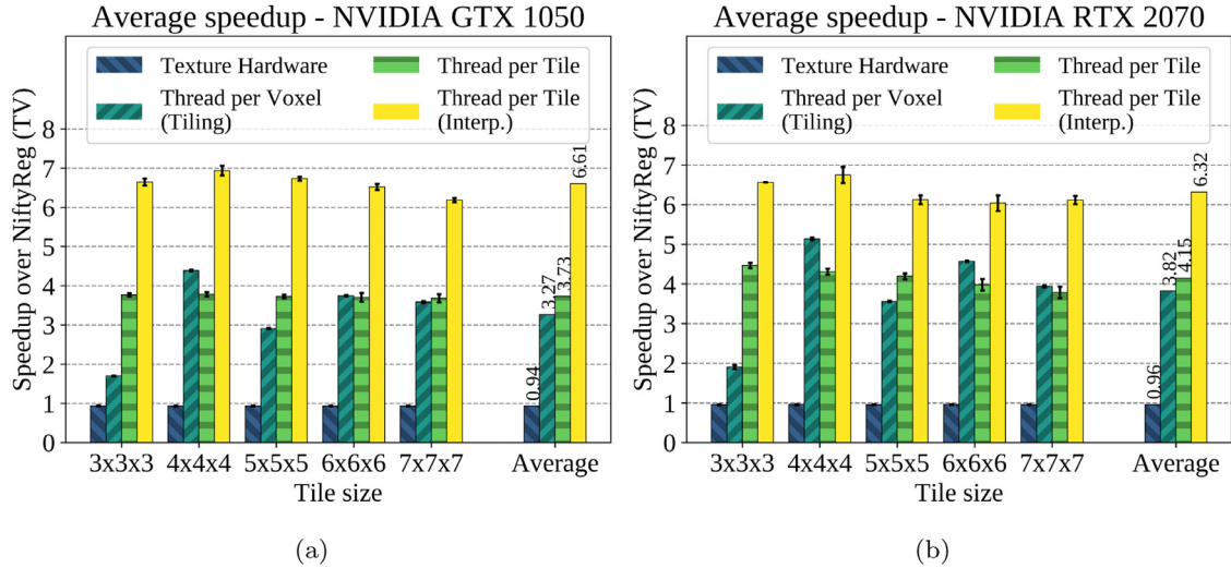
Fig. 6. Average speedup over NiftyReg (TV) for the five registration pairs with different tile sizes on the GTX 1050 GPU (a) and the RTX 2070 GPU (b). Error bars depict the standard deviation of the speedup.
