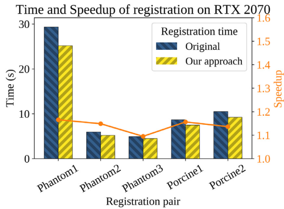
Fig. 9. Time and speedup of registration with our improved BSI GPU approach on RTX 2070.
