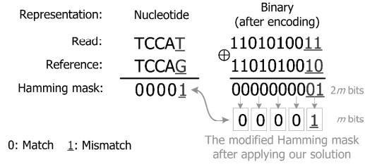
Fig. 3: An example of applying our solution for reducing the number of bits of each Hamming mask by half. We use a modified Hamming mask to store the result of applying bitwise OR operation to each two bits of the Hamming mask. The modified mask maintains the same meaning of the original Hamming mask.
