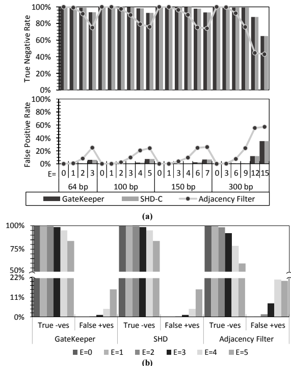
Fig. 5: Accuracy of GateKeeper, SHD, and the Adjacency Filter across different edit distance thresholds ( E ) and read lengths. We calculate the false positive [False +ves] and true negative [True -ves] rates using (a) simulated and (b) real mapping pairs.
