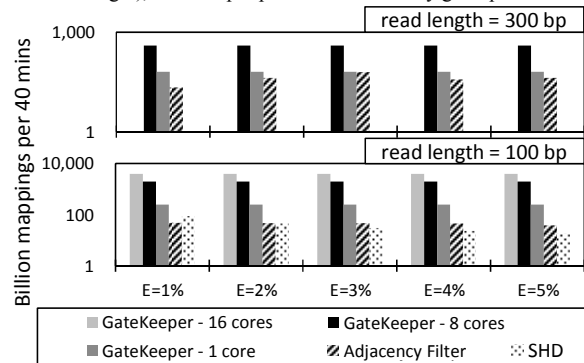
Fig. 4: The number of potential mappings for 100 and 300 bp long reads that are examined by GateKeeper, SHD, and the Adjacency Filter with different edit distance thresholds (y axis is on a logarithmic scale).
