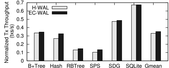
Fig. 7: Effect of Eager Commit on Transaction Throughput.
