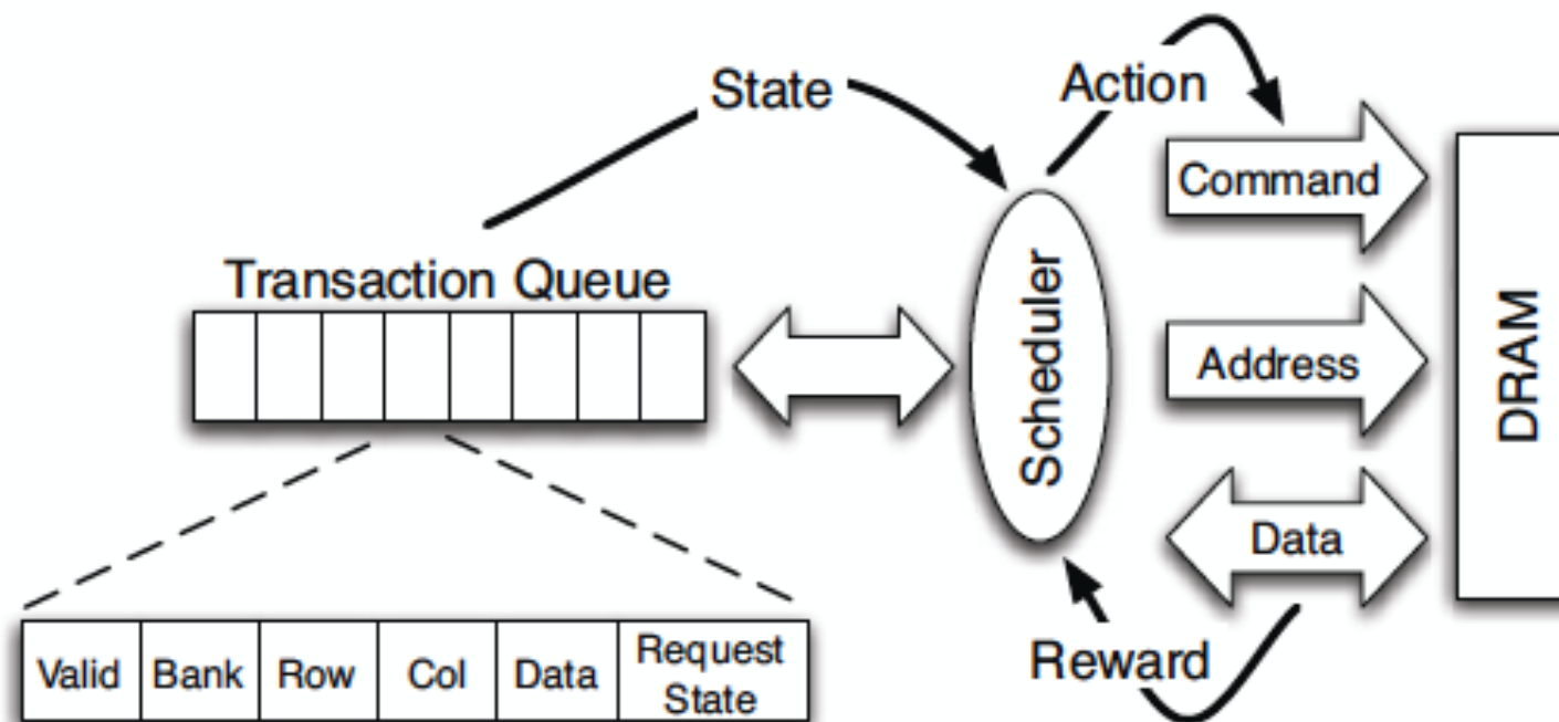
Figure 4: High-level overview of an RL-based scheduler.
