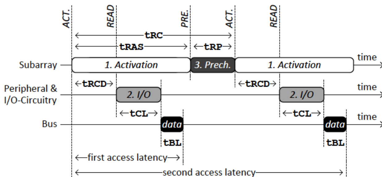
Figure 5. Three Phases of DRAM Access
