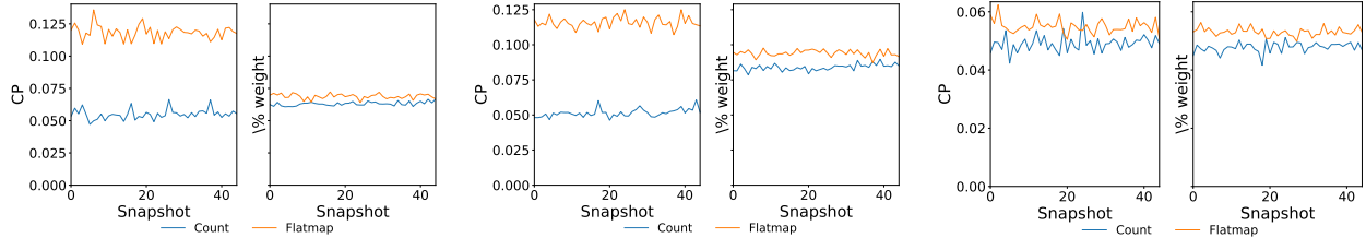
Figure 11: Operator and conventional profiling summaries for the benchmark of [18] on Flink and different configurations of operator parallelism. The source, flatmap, and count operators are configured with parallelism 4-2-4 (left), 1-2-4 (middle), and 4-4-4 (right).
