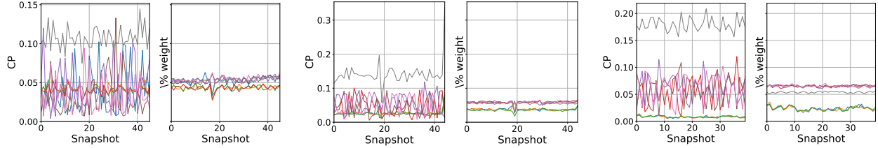
Figure 10: Straggler and conventional profiling summaries for the benchmark of [18] on Flink and different skewness percentage. The data generator has been configured with 30% (left), 50% (middle), and 80% (right) skewness.
