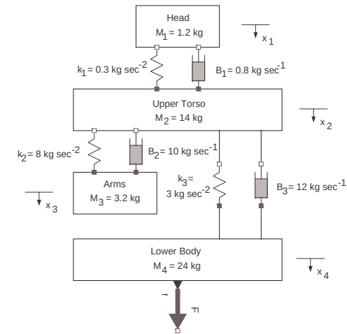
Figure: Mechanical model of a sitting human body
