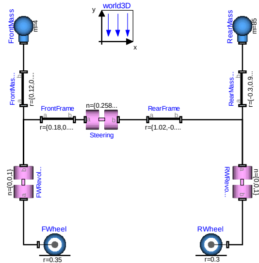
Figure 13: Multi-body diagram of a bicycle
