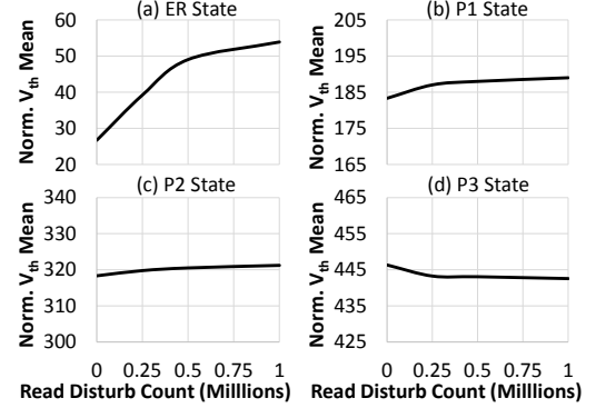
Fig. 4. Mean value of normalized cell threshold voltage, as the read disturb count increases over time. Distributions are separated by cell states.
