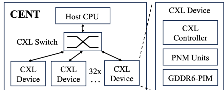
Figure 4. CENT Architecture.
