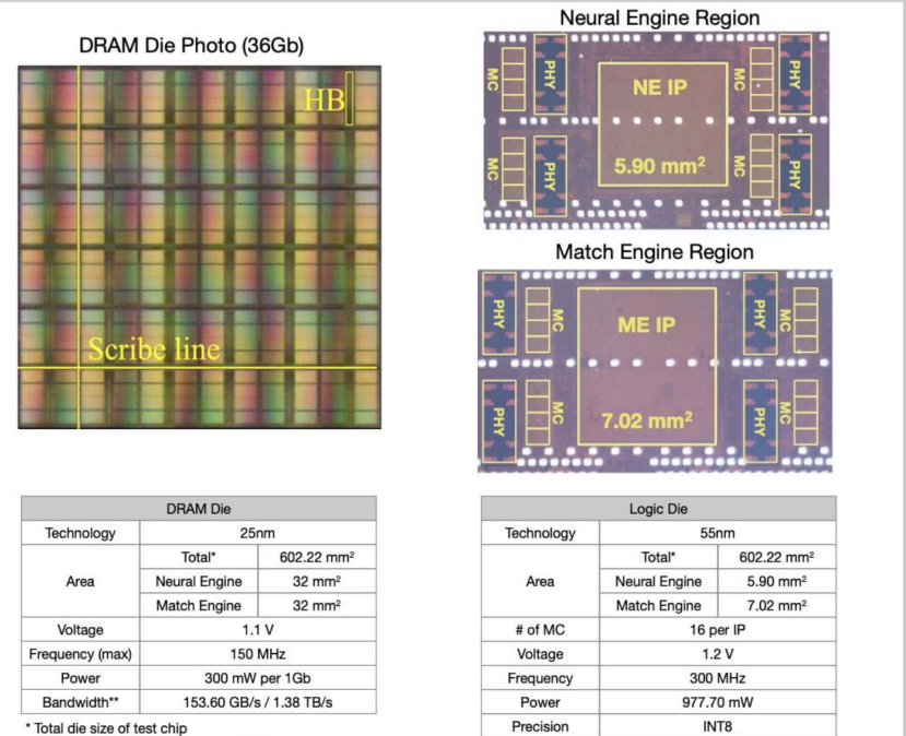
Figure 29.1.7: Die micrographs of DRAM die, NE and ME. Detailed specifications of DRAM die and logic die.
