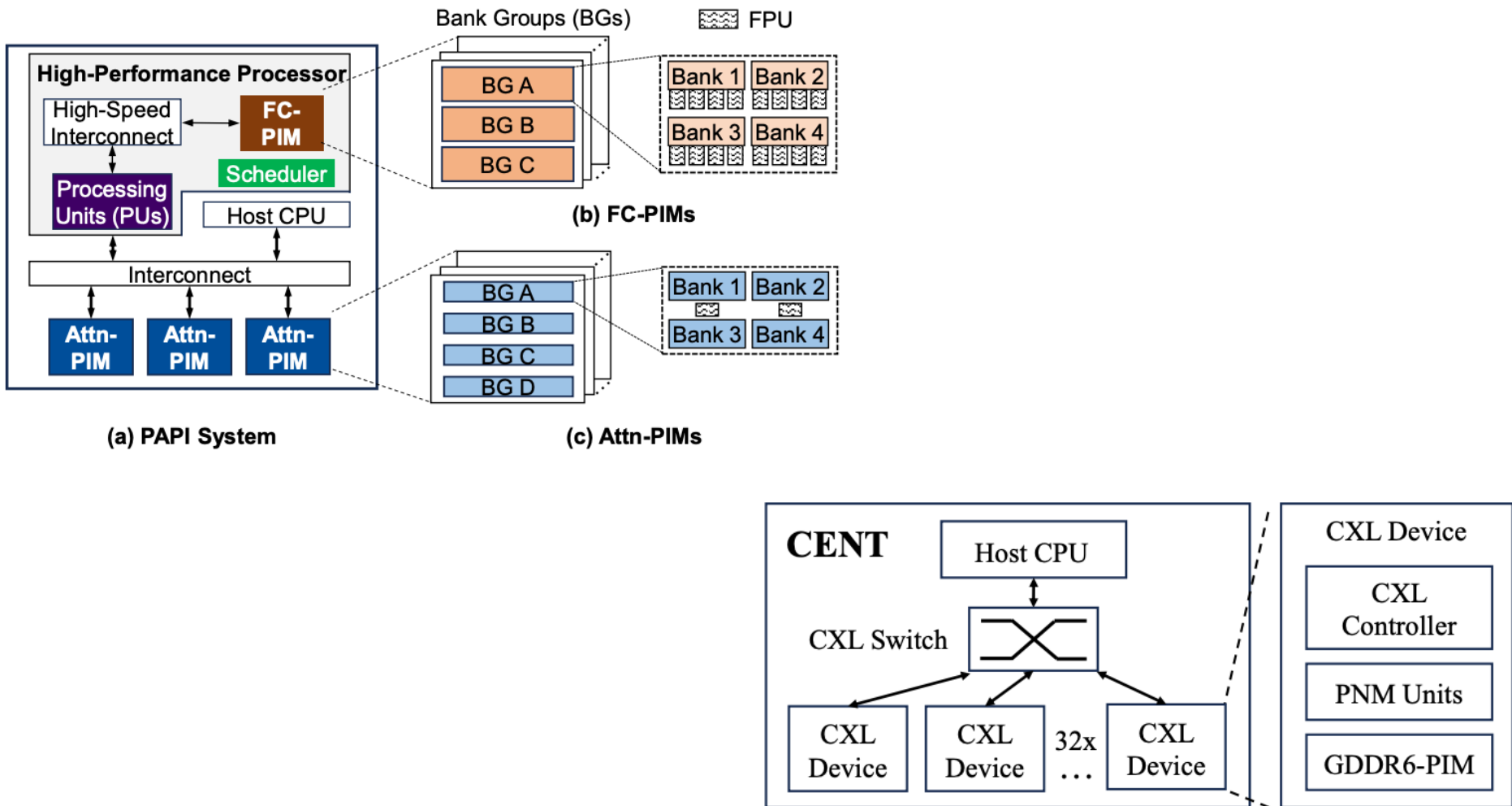
Figure 4. CENT Architecture.
